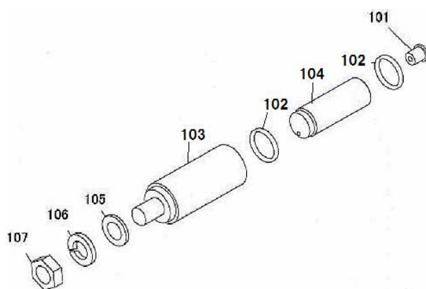
図番5-12-14(5-15-9)(6-3-14)(6-6-9) 爪外しシリンダAS
