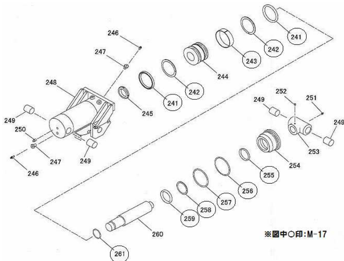
図番5-12-14(5-15-9)(6-3-14)(6-6-9) 爪外しシリンダAS
