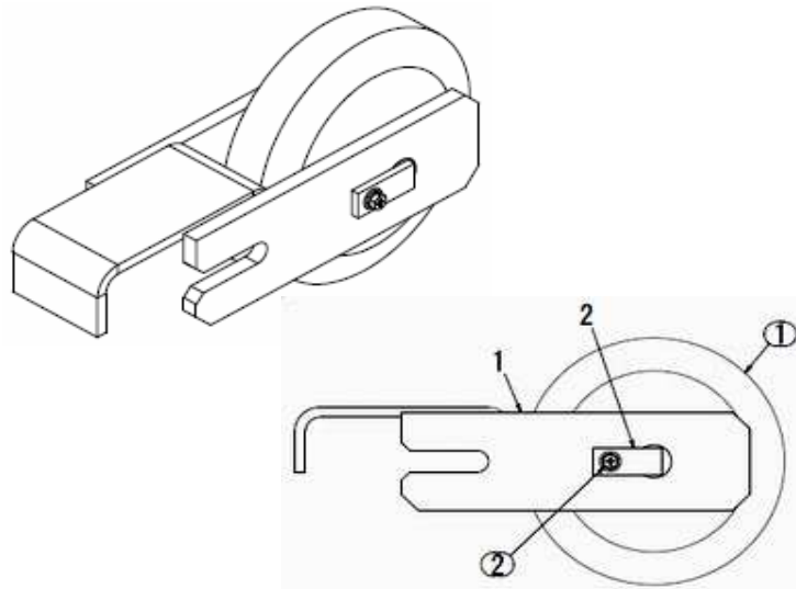
図番37 後輪 Bracket AS
