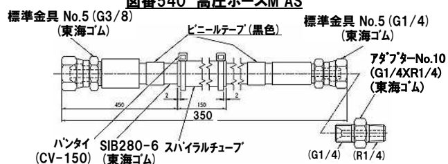
図番540 高圧ホースM AS
