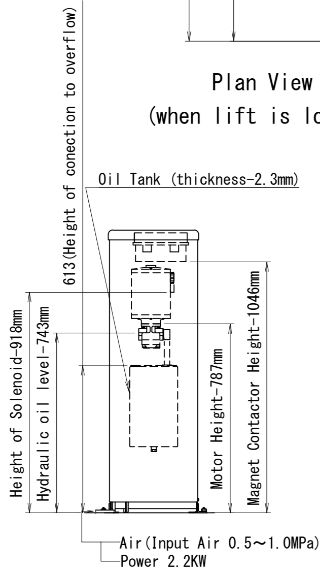
Hydraulic Unit
